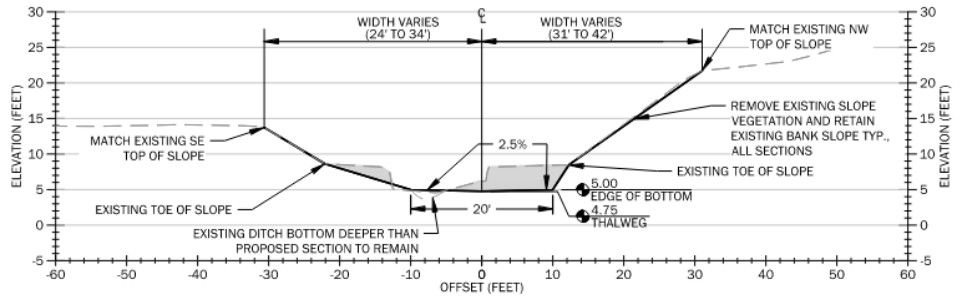
TYPICAL FIFE DITCH SECTION VIEW
